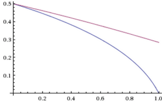
Figure 3: The degradation of the adversarial bound of Theorem 10 as f ranges in (0, 1) in the x-axis (lower curve). When ties are broken following lexicographic order the analysis can be improved (upper curve).
